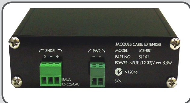
JCE-8B1 rear
